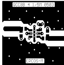
Optimised PCB layout for SAW filters in QCC8B package, pinning 1,5 (top side, scale 1:1)
