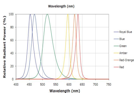
Wavelength characteristics
