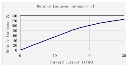
Light intensity and forward current curves
