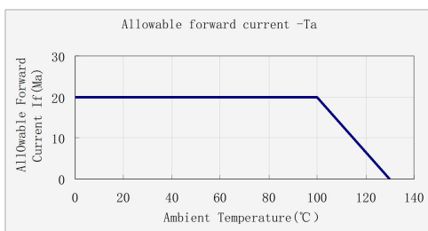
Maximum Forward DC vs. Temperature Graph
