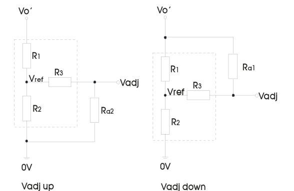
Applied circuits of Vadj (Part in broken line is the interior of models)
