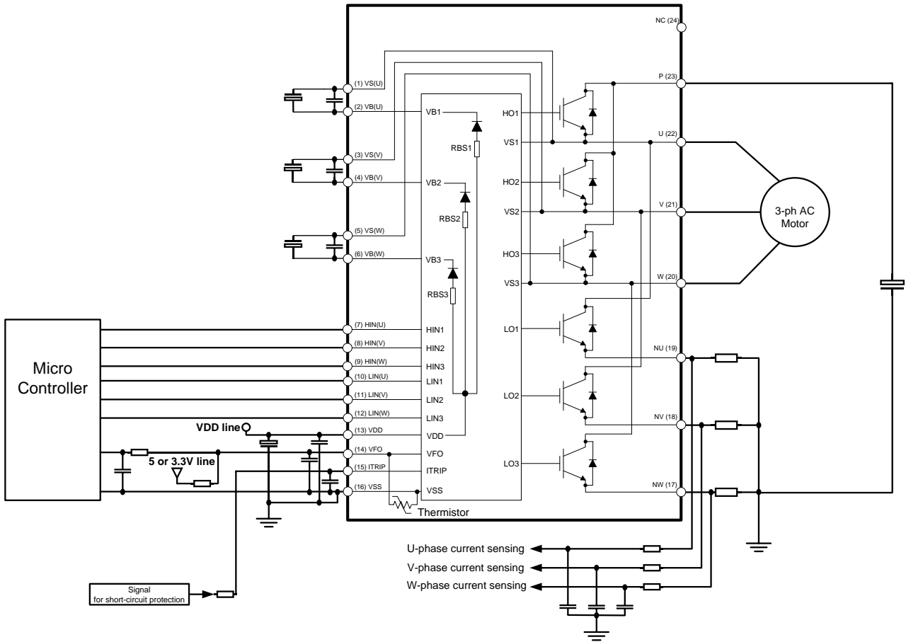
Figure 9: Application circuit
