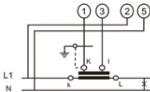
Single phase
