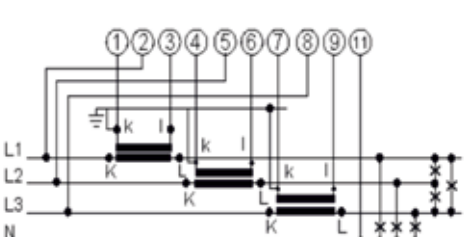
3-phase 4 wire unbalanced load
