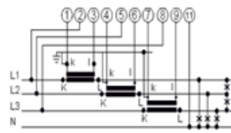
3-phase 4 wire unbalanced load
