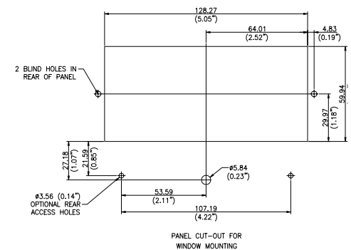
Window mount cut-out
