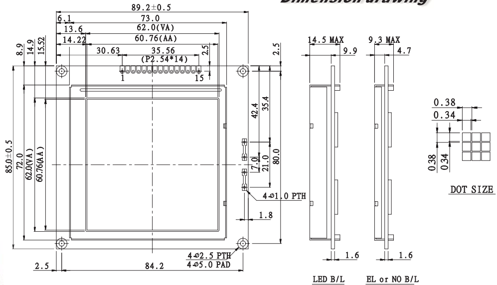
Dimension drawing
